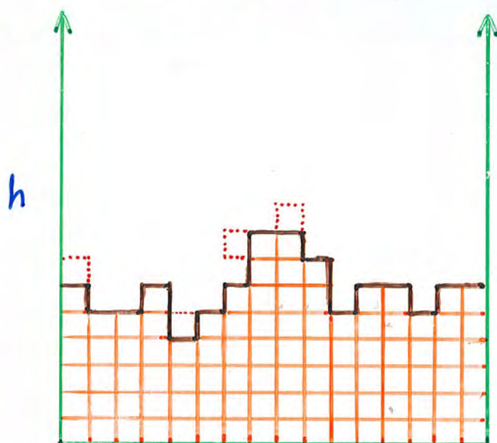
EDEN MODEL
