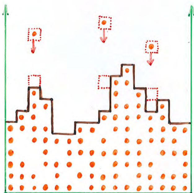
BALLISTIC DEPOSITION
