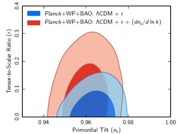
Fig. 4. Marginalized joint 68% and 95% CL regions for (r, n_s) , using \text{Planck}+\text{WP}+\text{BAO} with and without a running spectral index.
