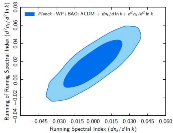
Fig. 3. Marginalized joint 68% and 95% CL regions for (d^2 n_s/d^2 \ln k, dn_s/d \ln k) using \text{Planck}+\text{WP}+\text{BAO} .
