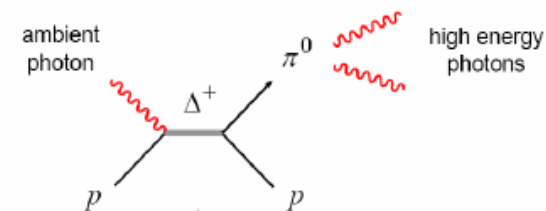
proton acceleration
