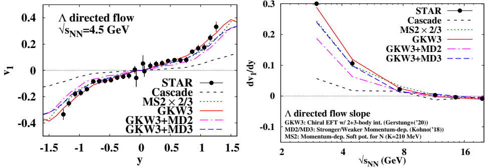
Figure 2. Left: Calculated directed flow of \Lambda in mid-central Au + Au collisions at \sqrt{s_{NN}} = 4.5 GeV. Right: The directed flow slope of \Lambda . Data are taken from Ref. [7].
