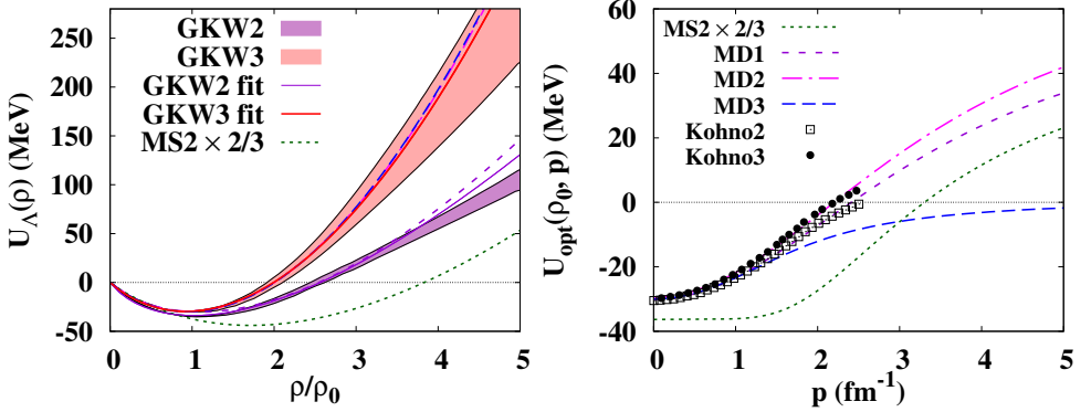
Figure 1. Baryon-density (left) and momentum (right) dependence of the single-particle potentials for \Lambda . GKW2 and GKW3 represent the \Lambda single-particle potential from \chi EFT with 2- and 2+3-body interactions [3]. MS2 \times 2/3 shows the nucleon single-particle potential multiplied by 2/3. MD1, MD2, and MD3 are momentum-dependent potentials obtained by fitting the \chi EFT results [4].
