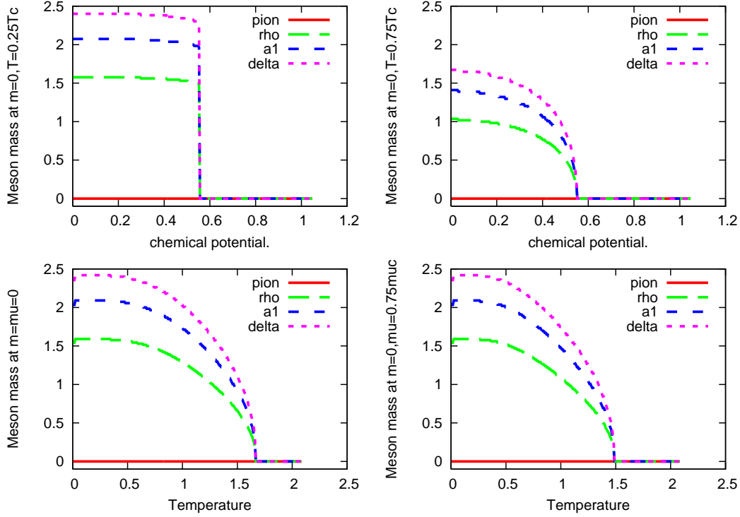
Figure 1: The \mu dependence of meson mass at T = 0.25T_c(\mu = 0) (:upper-left) and T = 0.75T_c(\mu = 0) (:upper-right). T dependence of meson mass at \mu = 0 (:lower-left) and \mu = 0.75\mu_c(T = 0) (:lower-right). From 3.7. We are considering the chiral limit case in the lattice unit.
