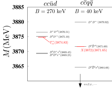
Fig. 1. Thresholds related to T_{cc}^+ and X(3872) , which are located 270 keV and 40 keV below the D^0D^{*+} and D^0\bar{D}^{*0} thresholds, respectively.
