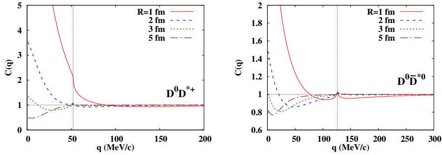
Fig. 2. The correlation functions of the D^0D^{*+} (left) and the D^0\bar{D}^{*0} (right) pairs with the source size R = 1, 2, 3, and 5 fm.
