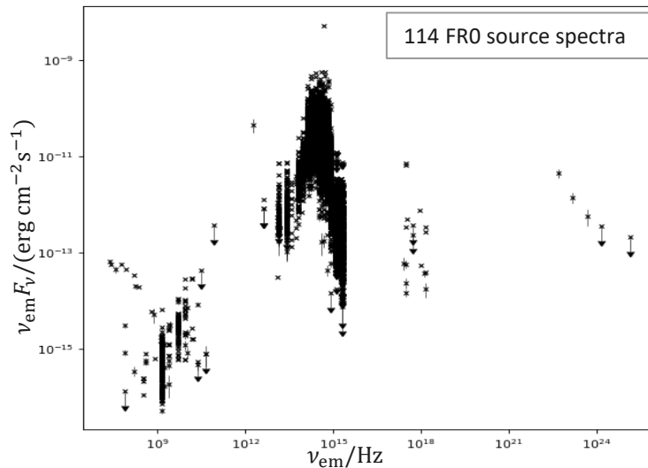
Spectral energy distribution
