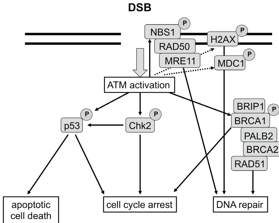
Figure 3. Key players of the DNA damage response signaling pathways
