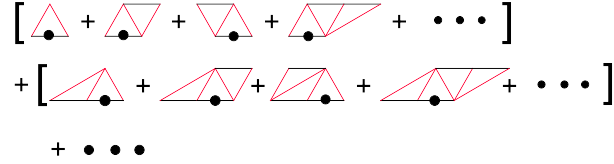
Figure 27: The combinatric calculus of the generating function for the one-step-propagator from the combinatorics:
