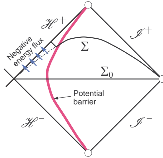
図 6.11: Flux integral to estimate the growth rate
