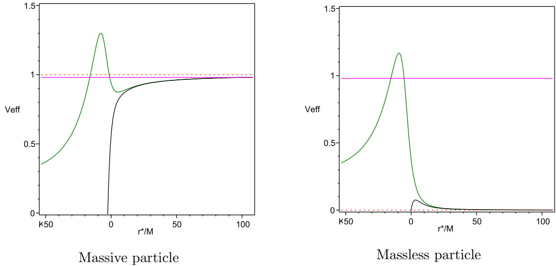
図 6.6: The effective potential for particles with L = 3 (corotating) and L = -3 (counter-rotating) around the Kerr BH with a = 0.999 . r^* is the tortoise coordinate defined by dr^* = (r^2 + a^2)dr/\Delta .
