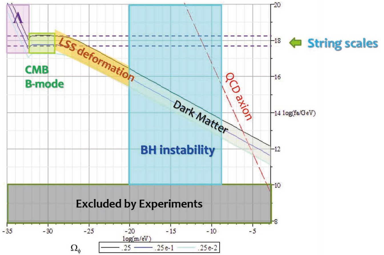
図 5.2: Axion abundance and relevant phenomena
