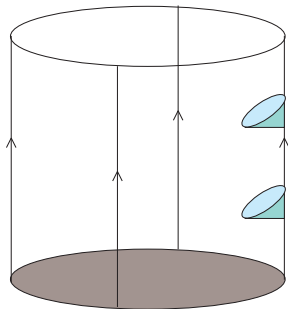
図 6.2: Killing horizon
