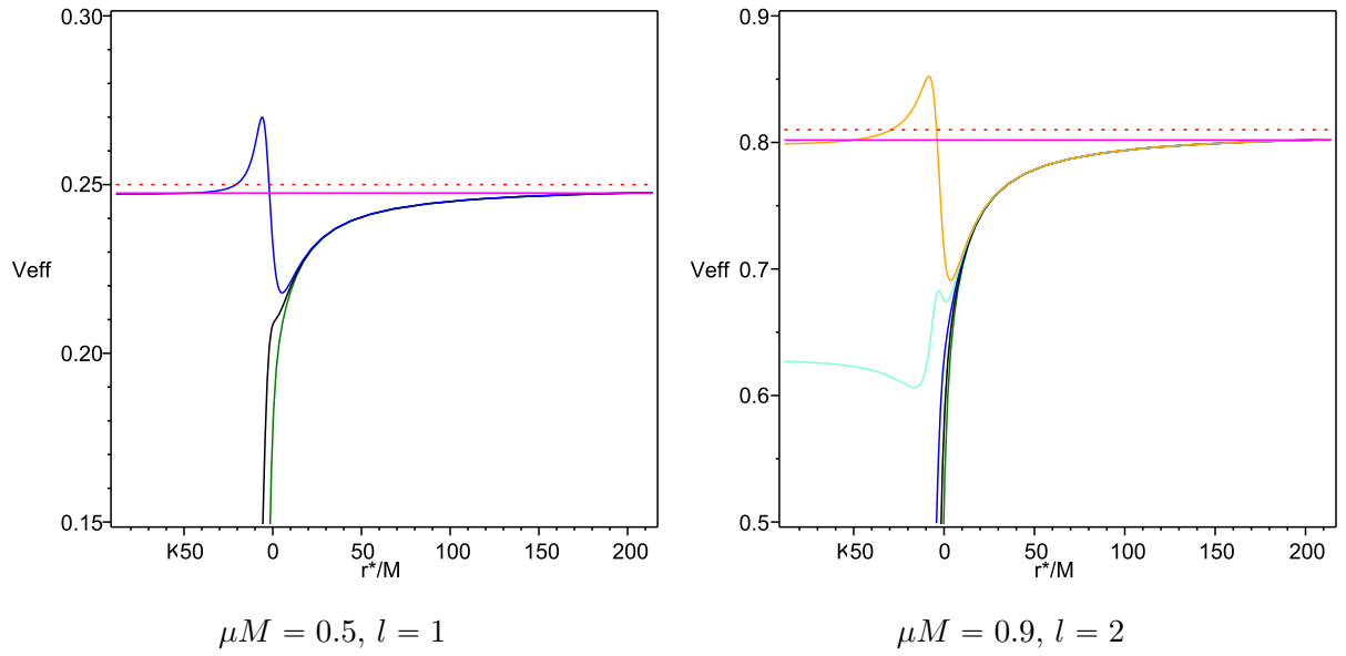
図 6.9: The effective potential for a massive scalar field around the Kerr BH with a = 0.999 .
