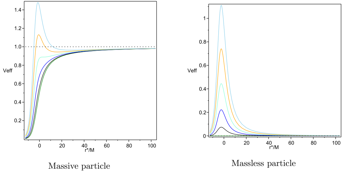
図 6.5: The effective potential for a particle with L = 0, \dots, 5 around the 4D Schwarzschild BH
