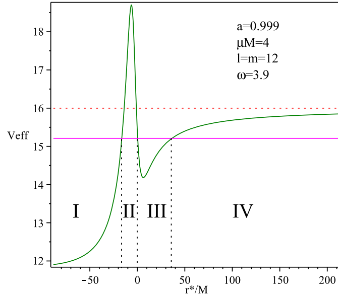
図 6.10: Division into four regions for the WKB approximation
