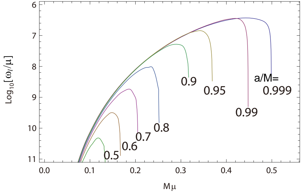
図 6.12: The instability growth rate for l = m = 1 .
