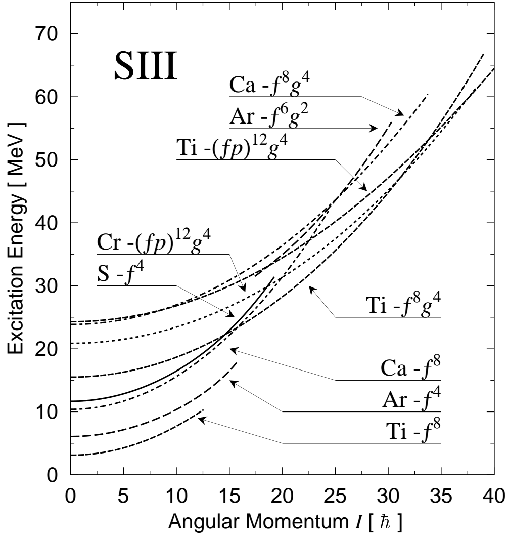
Figure 4: Excitation energy vs. angular-momentum plot for the SD and HD rotational bands obtained by the cranked SHF calculations with the use of the SIII interaction. Their configurations are indicated by the same notations as in Fig. 1.
