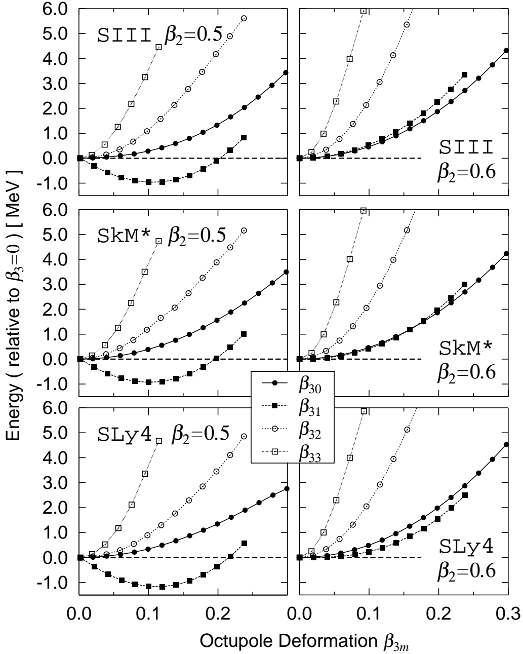
Figure 13: Left-hand side: Deformation energy curves (measured from energies at \beta_3 = 0 ) as functions of the octupole deformation parameters \beta_{3m} ( m = 0, 1, 2, 3 ), calculated for ^{40}\text{Ca} by means of the constrained HF procedure. The quadrupole deformation parameters are fixed at \beta_2 = 0.5 and \gamma = 0 . One of the \beta_{3m} ( m = 0, 1, 2, 3 ) is varied while the other \beta_{3m} 's are fixed to zero. Right-hand side: The same as the left-hand side, except that the quadrupole deformation parameters are fixed at \beta_2 = 0.6 and \gamma = 0 . Results of calculation with the use of the SIII, SkM*, and SLy4 interactions are displayed in the upper, middle and lower panels, respectively.
