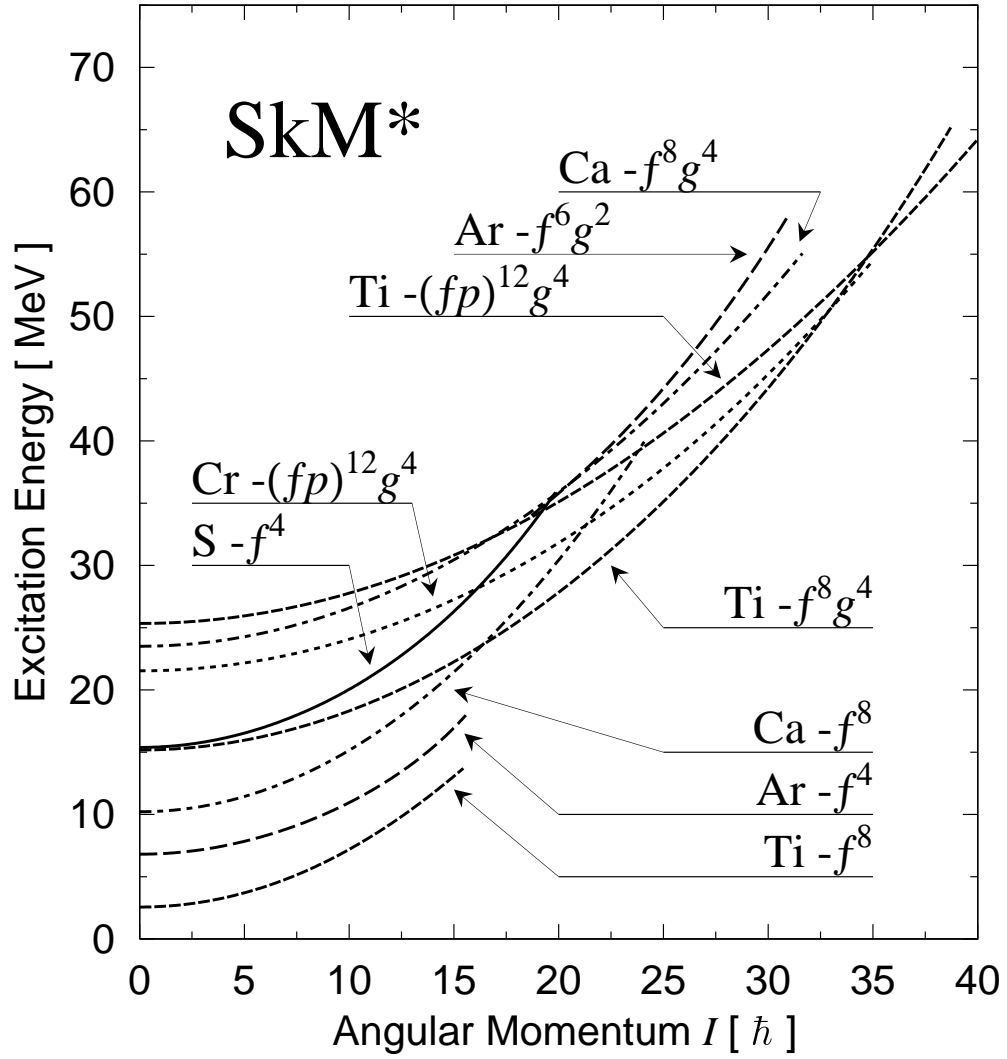
Figure 5: The same as Fig.4 but for the SkM* interaction.
