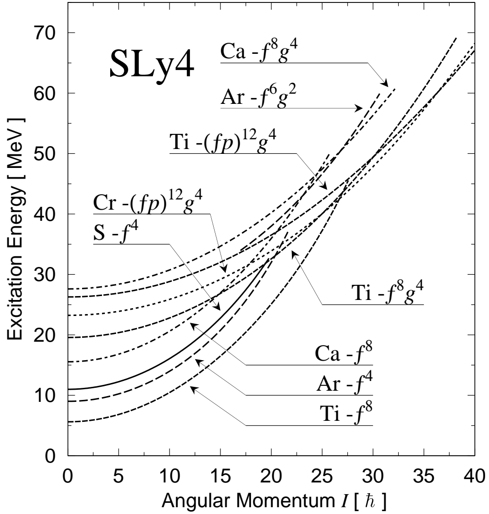
Figure 6: The same as Fig.4 but for the SLy4 interaction.
