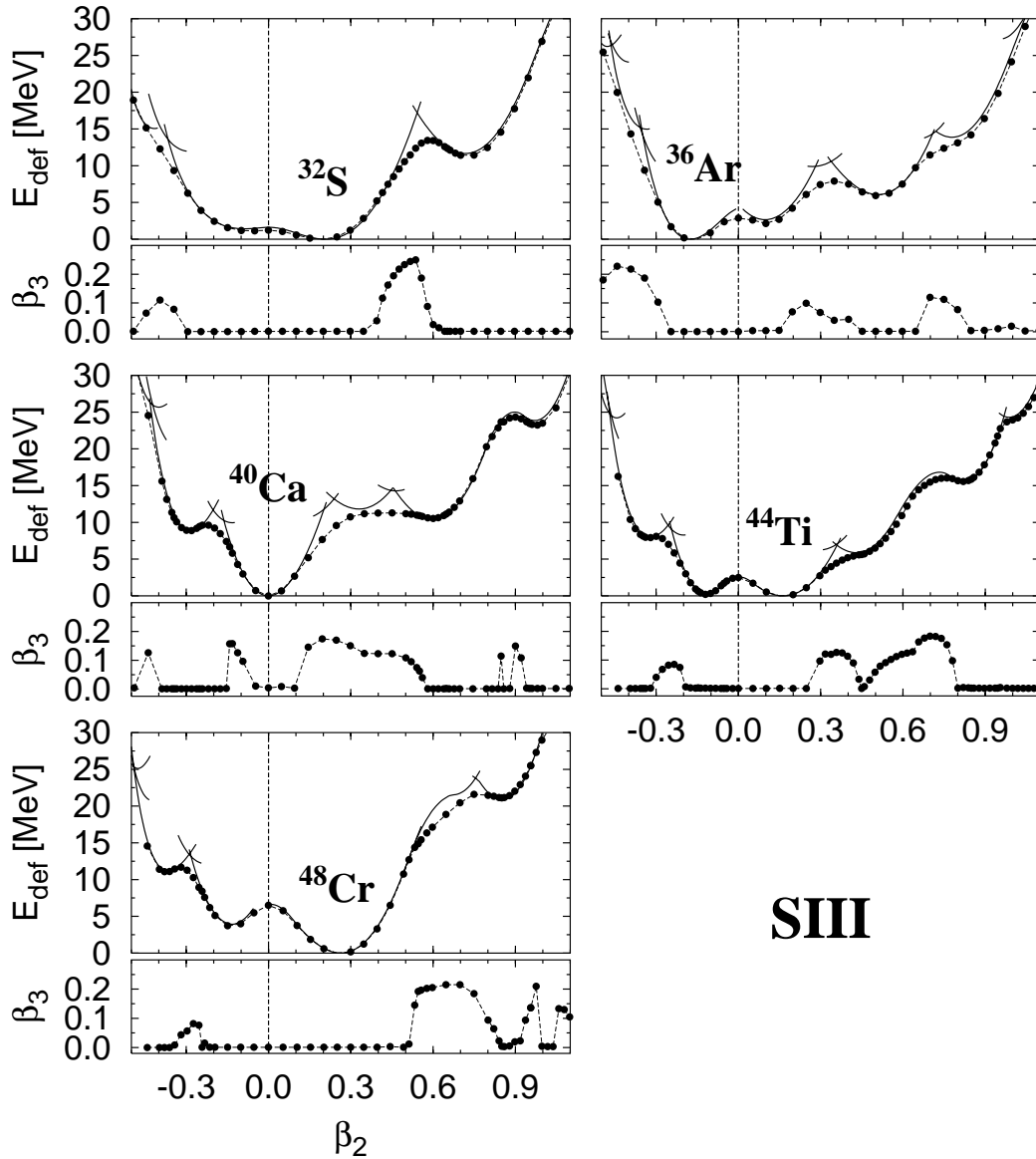
Figure 10: Octupole deformation parameters \beta_3 of the lowest energy states for given values of \beta_2 , obtained by the unrestricted SHF calculation at I = 0 with the use of the SIII interaction. Their values are plotted as functions of \beta_2 in the lower portion of each panel. To show that their values increase at crossing regions between configurations involving different number of particles in the fp shell, the deformation energy curves are also displayed in the upper portion of each panel. The latter are the same as those presented in Fig. 1.
