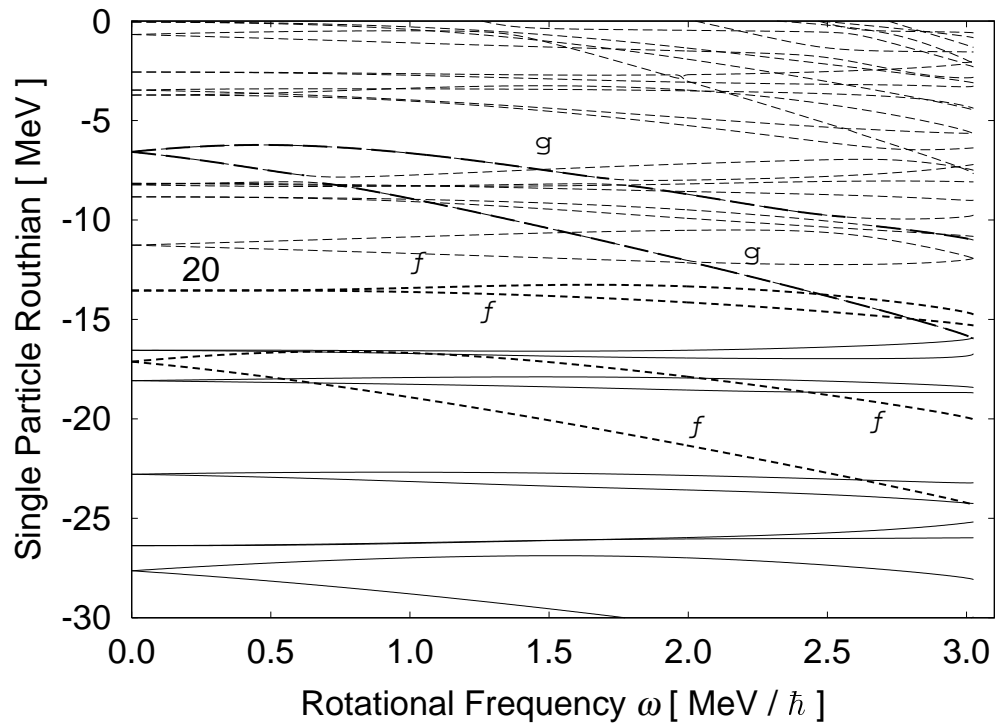
Figure 8: Neutron single-particle energy diagram (Routhian) for the SD band in ^{40}\text{Ca} , calculated with the use of the SIII interaction and plotted as functions of rotational frequency \omega_{\text{rot}} . The levels associated with the f_{7/2} and g_{9/2} shells are drawn by thick-broken and long-dashed lines, respectively.
