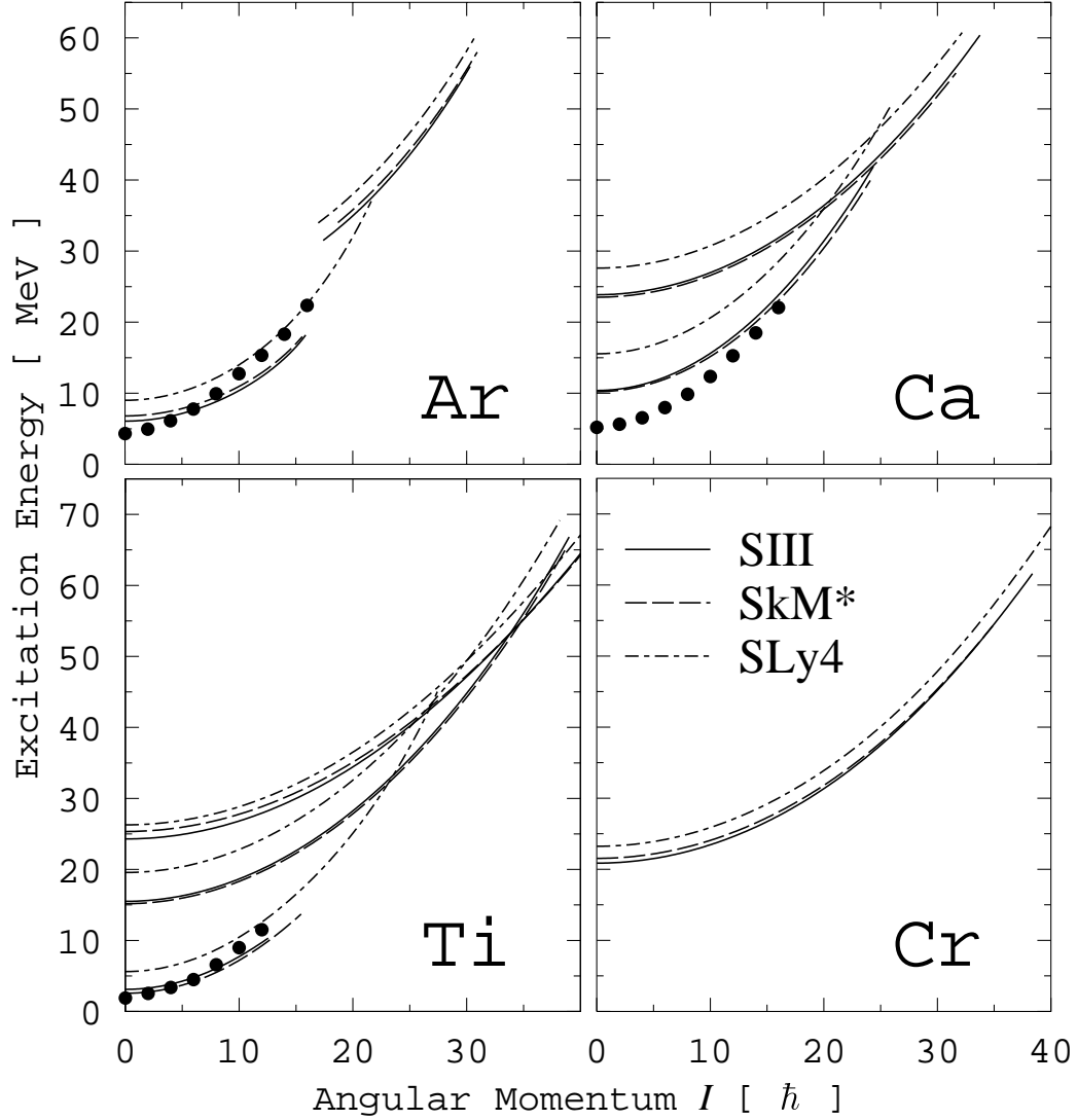
Figure 9: Comparison between the excitation energies of the SD and HD bands in ^{36}\text{Ar} , ^{40}\text{Ca} , ^{44}\text{Ti} and ^{48}\text{Cr} , calculated by using different versions of the Skyrme interaction and the experimental data ( [16] for ^{36}\text{Ar} , [19] for ^{40}\text{Ca} , and [20] for ^{44}\text{Ti} ). The data are shown by filled circles and the results with the SIII, SkM* and SLy4 interactions are drawn by solid, dashed and dashed-dotted lines, respectively.
