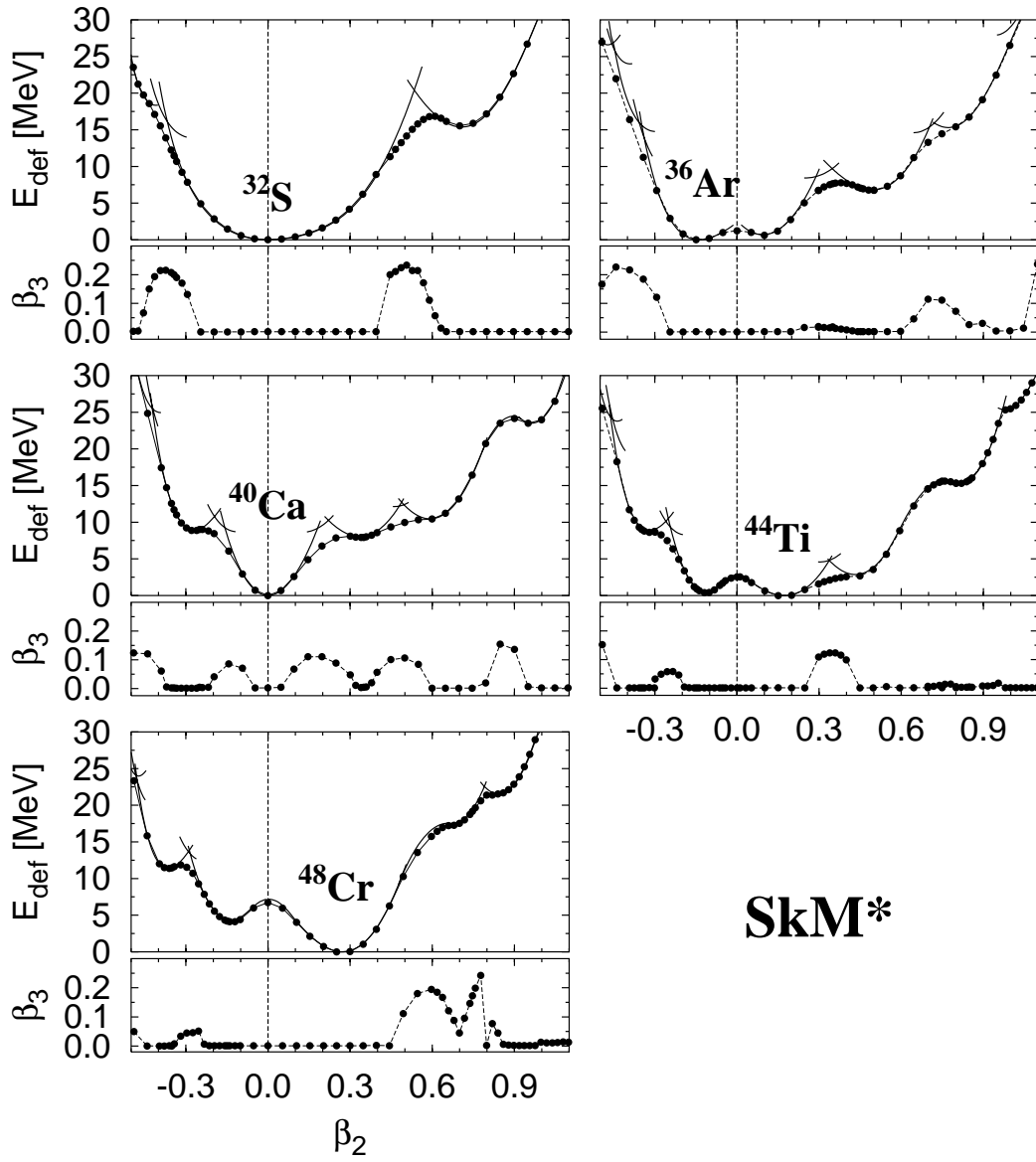
Figure 11: The same as Fig.10 but for the SkM* interaction.
