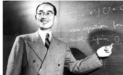
Yukawa
