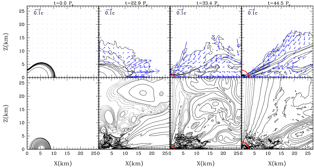
FIG. 1 (color online). Upper four panels: Snapshots of the density contours for \rho (solid curves) and velocity vectors. The contours are drawn for \rho = 10^{15-0.4i} \text{ g/cm}^3 ( i = 0-9 ). In the last panel, a curve with \rho = 10^{11} \text{ g/cm}^3 is also drawn. The (red) circle near the center in the last two panels denotes an apparent horizon. The scale of the velocity is indicated in the upper left corner. The lower four panels denote the magnetic field (contours of the toroidal component of the vector potential A_\varphi ) at the same times as the upper panels. The solid contour curves are drawn for A_\varphi = 0.8(1-0.1i)A_{\varphi,\text{max},0} ( i = 0-9 ) and the dotted curves are for A_\varphi = 0.08(1-0.2i)A_{\varphi,\text{max},0} ( i = 1-4 ). Here, A_\varphi = A_{\varphi,\text{max},0} is the maximum value of A_\varphi at t = 0 .
