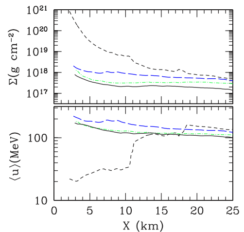
FIG. 2 (color online). Evolution of the surface density and averaged thermal energy per nucleon of the torus as functions of cylindrical radius at t/P_c = 33.4 (dashed curves), 39.3 (long-dashed curves), 44.5 (dotted-dashed curves), and 49.9 (solid curves).
