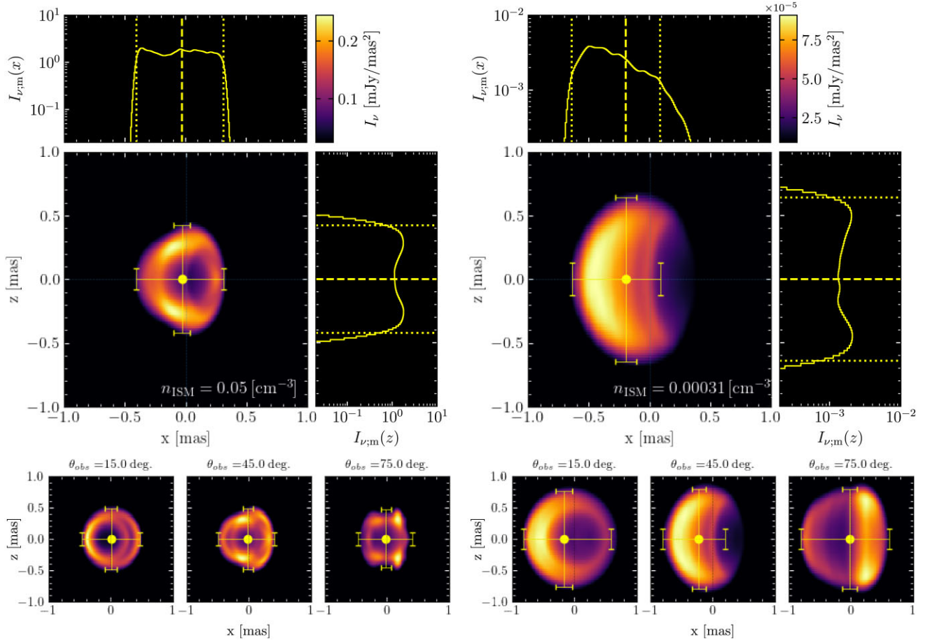
Figure 1. Top figure: sky map for a BNS merger simulation with BLh EOS and q = 1.00 computed at 120 d, after the merger at \nu = 1 GHz, and observed at \theta_{\text{obs}} = 45^\circ . Left and right columns of plots corresponds to different ISM densities, n_{\text{ISM}} = 0.05 \text{ cm}^{-3} on the left and n_{\text{ISM}} = 0.00031 \text{ cm}^{-3} on the right. In each plot column, the top and top-right subplots display the X and Z averaged brightness distributions, respectively. Dotted lines mark FWHM and dashed lines mark the location of the flux centroid of the image. FWHM and the location of the flux centroid are also shown on the main panel of the figure as error bars and the circular marker, respectively. Thin grey dotted lines indicate the X - and Z -axis. Notably, we are plotting I_\nu/I_{\nu,\text{max}} \in (0.1, 1) range of the normalized specific intensity in order to resolve the image structure more clearly. Bottom panel: same sky map but viewed at three difference angles, \theta_{\text{obs}} .
