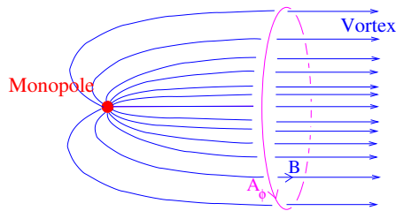
Fig. 1. A monopole-vortex system
