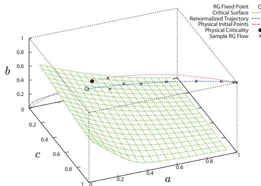
Figure 1: Phase structure of DWRGT
