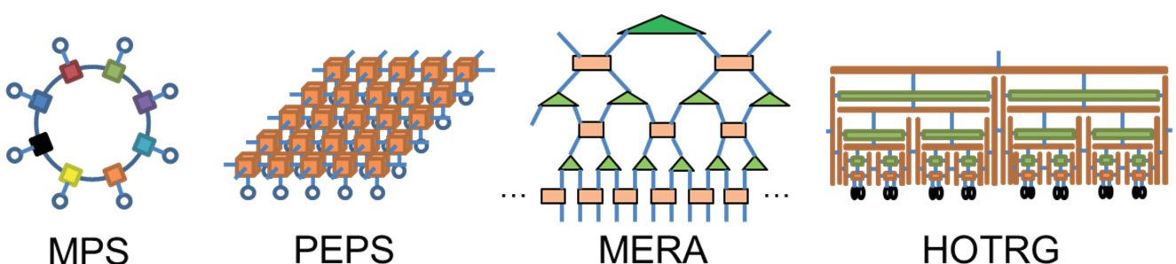
Fig. 1: Typical examples of tensor network diagrams
