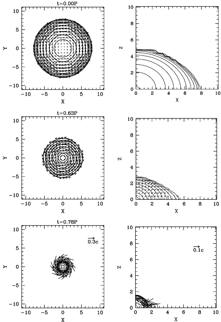
FIG. 9. Same as Fig. 6, but for star (A) with \Delta K/K = 10\% . The contour lines are drawn for \rho_*/\rho_{*c} = 10^{-0.3j} for j=0,1,2,\dots,10 where \rho_{*c} is 0.012, 0.20, and 1.01 for the three different times.
