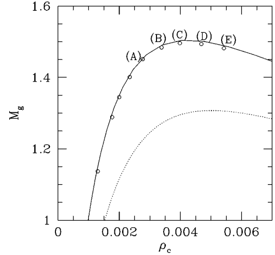
FIG. 1. The gravitational mass M_g as a function of the central density \rho_c for rotating stars with \Gamma=2 and K=200/\pi . The solid and dashed lines denote exact solutions for sequences of rotating stars at the mass-shedding limit and spherical stars. The open circles denote the sequence of rotating stars at the mass-shedding limit as obtained from the conformal flatness approximation. The configurations that we adopt as initial data for dynamical evolution calculations in this paper are marked with (A)–(E).
