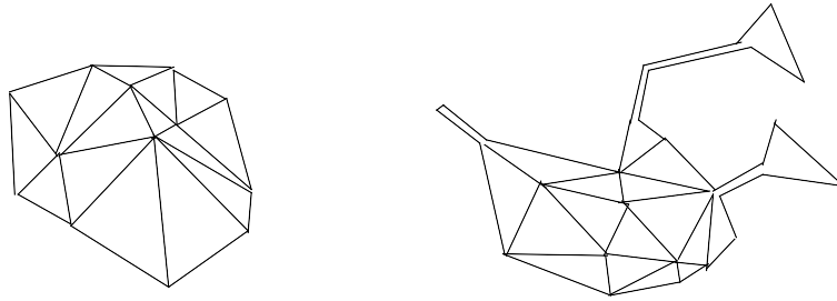
Figure 9: Randomly triangulated surfaces: The left is the regular triangulation, and the right is the unrestricted triangulation.
