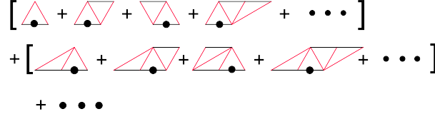
Figure 27: The combinatoric calculus of the generating function for the one-step-propagator
