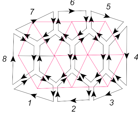
Figure 15: The triangulated surface with one boundary
