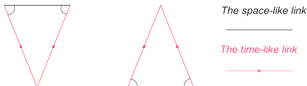
Figure 22: Simplices in the causal dynamical triangulation
