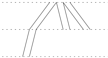
Figure 19: UURRURUR-type branched polymer with 2l = 8
