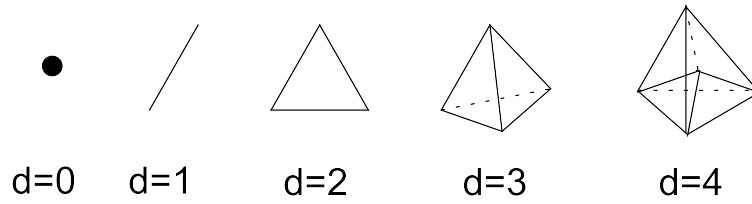
Figure 36: Simplicies in several dimensions
