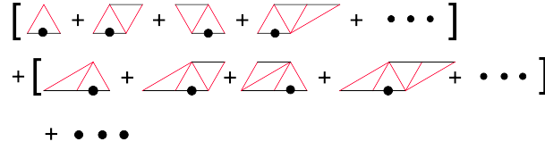
Figure 27: The combinatric calculus of the generating function for the one-step-propagator
