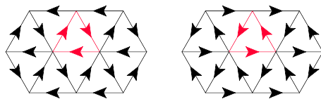
Figure 13: The orientation of the triangulated surface
