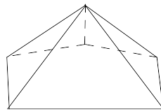
Figure 8: N_i < 6
