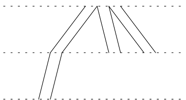
Figure 19: UURRURUR-type branched polymer with 2l = 8
