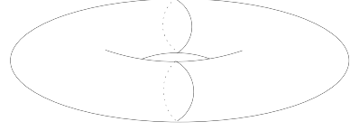
Figure 5: The surface with uncontractible boundary loops
