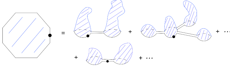
Figure 10: All possible triangulations with one boundary: one of boundary links is marked by a point.
