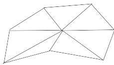
Figure 7: N_i > 6
